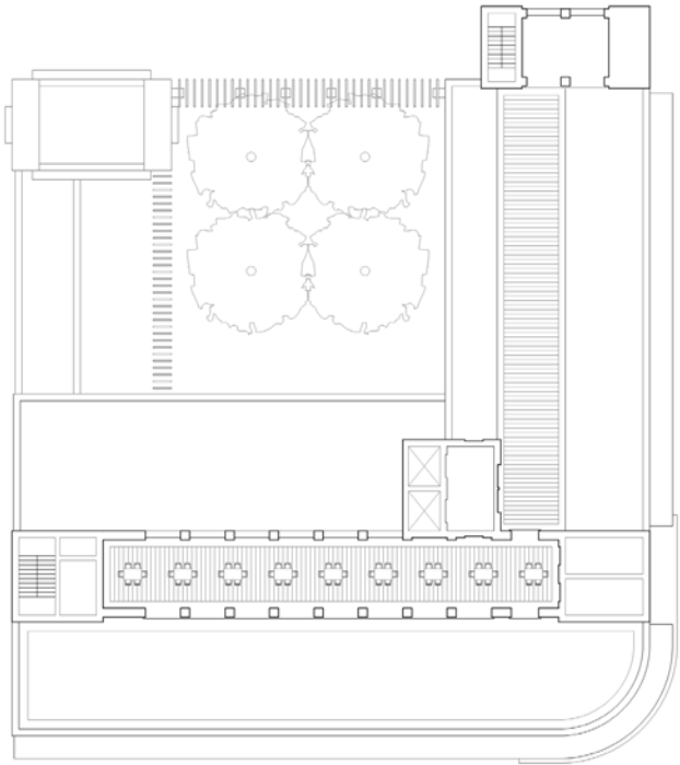
Roof plan.
