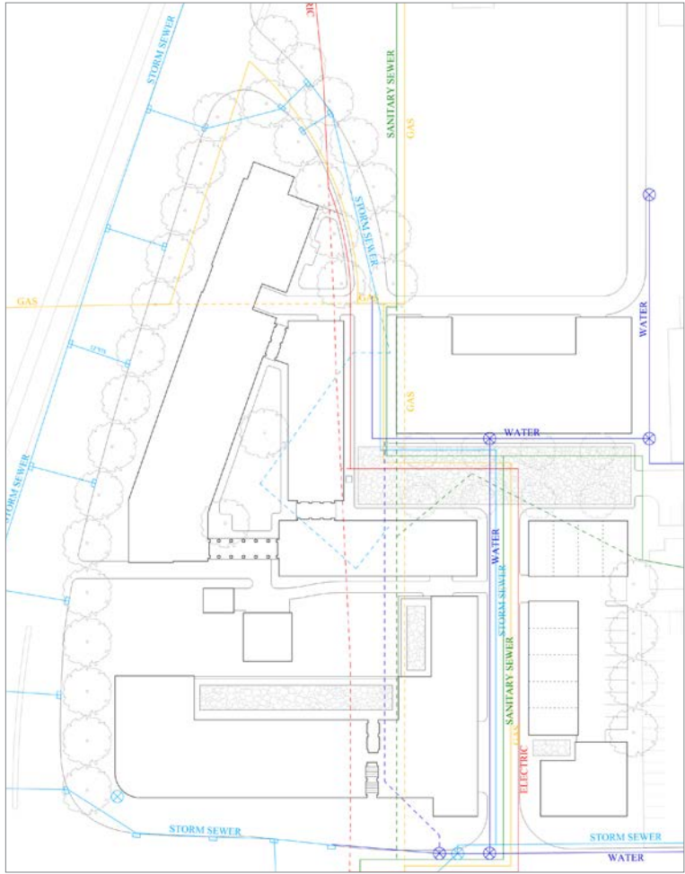
Utilities diagram.
