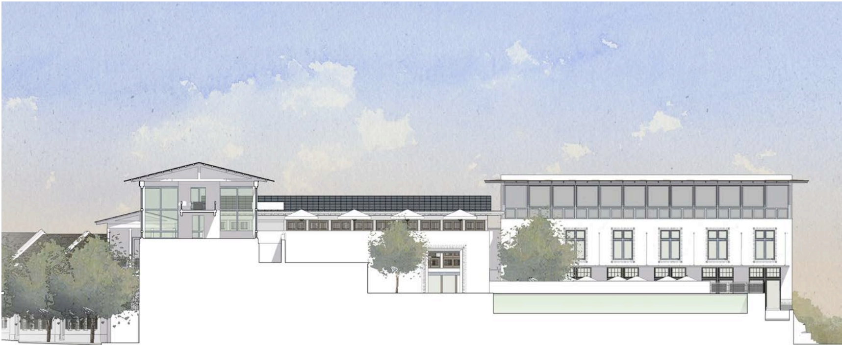
E-W section looking north.
